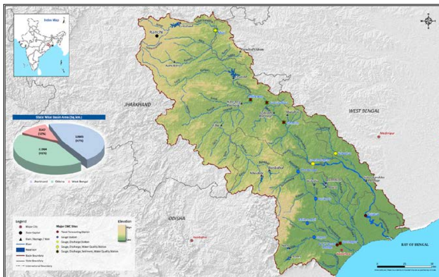
Figure 12: Subernarekha and Burhabalang River Basin.
