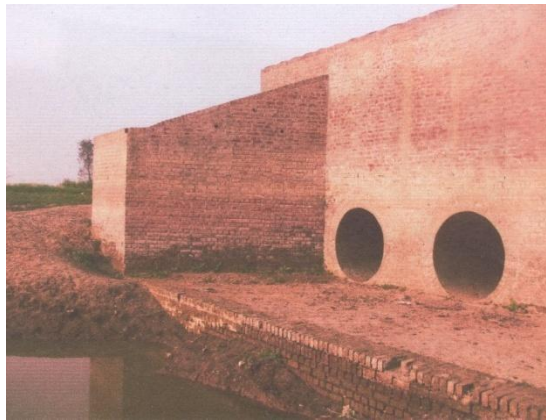
Figure 7-1: A cross drainage work
