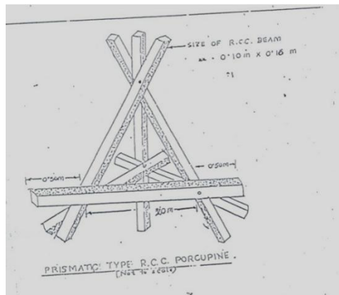
Figure 2-3: A sketch of typical RCC porcupine
