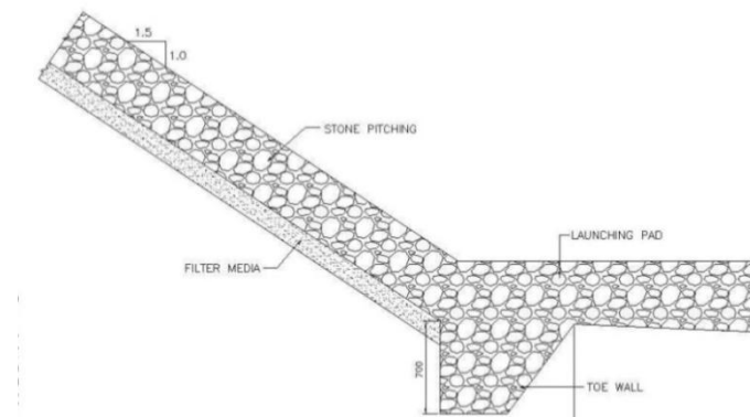
Figure 4-14: Toe protection using toe wall and apron
