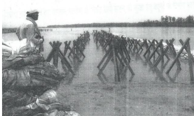
Figure 5-8: A typical RCC porcupine spur
