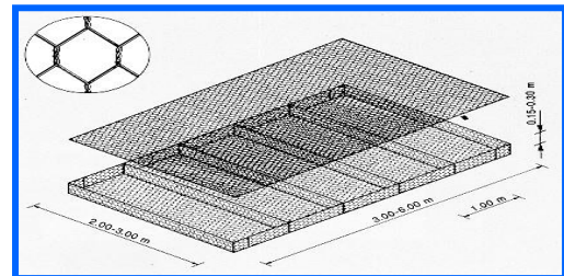
Figure 2-2: Hexagonal double twist steel wire mesh, revet-mattress
