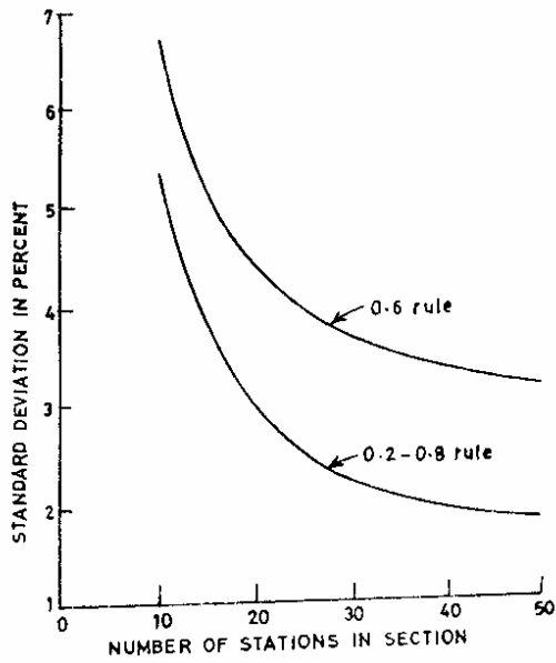
Fig. 2: Standard Deviation of Total Error of Discharge Measurements (Modified from Carter 1973)
