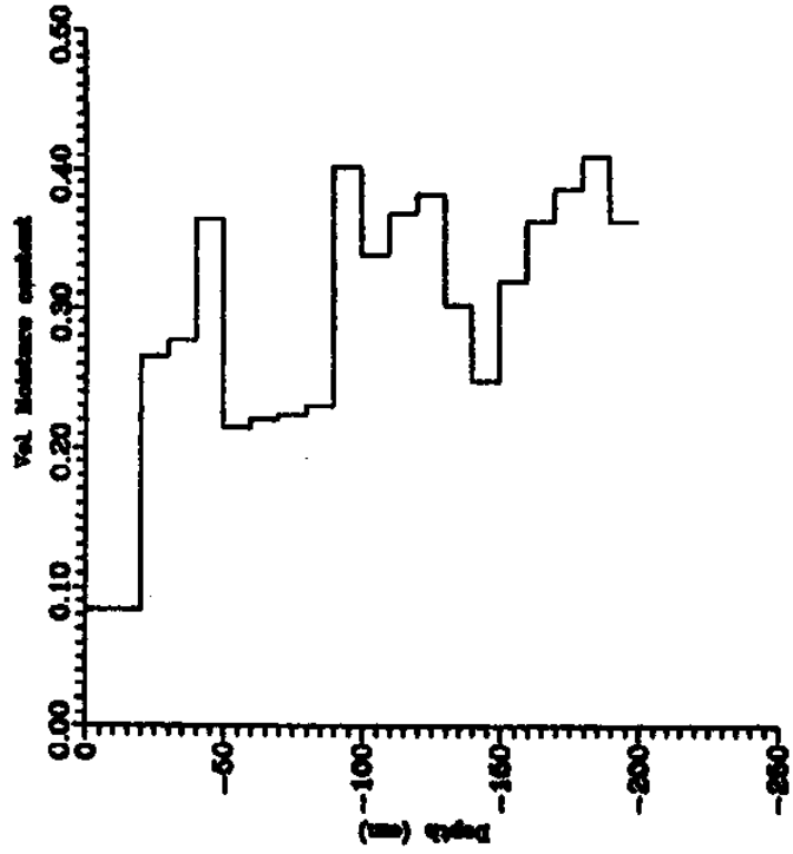
Fig. 9 : Movement of Injected Tritium and Soil Moisture at Surwari site
