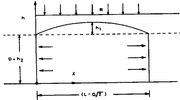
Fig. 2 Problem definition of the horizontal flow
