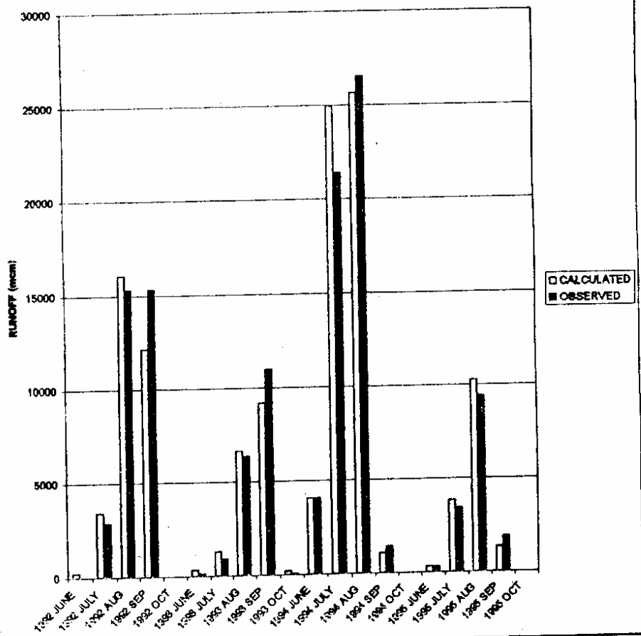
FIG. 21: COMPARISON OF MONTHLY CALCULATED AND OBSERVED SURFACE RUNOFF FOR BEARMA AT GARSABAD G.D. SITE
