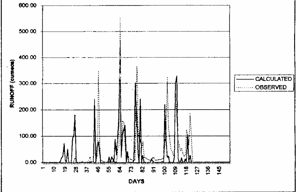
FIG. 18: COMPARISON OF CALCULATED AND OBSERVED SURFACE RUNOFF FOR SONAR AT GARHAKOTA G.D. SITE (JUNE TO OCT. 1993)
