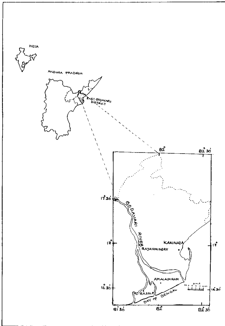
Fig. 2 Location of the study area
