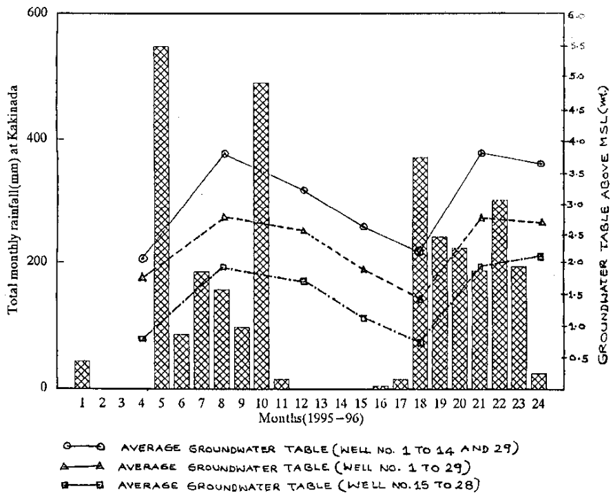
FIGURE 6 COMPARISON BETWEEN RAINFALL AND AVERAGE GROUNDWATER TABLE
