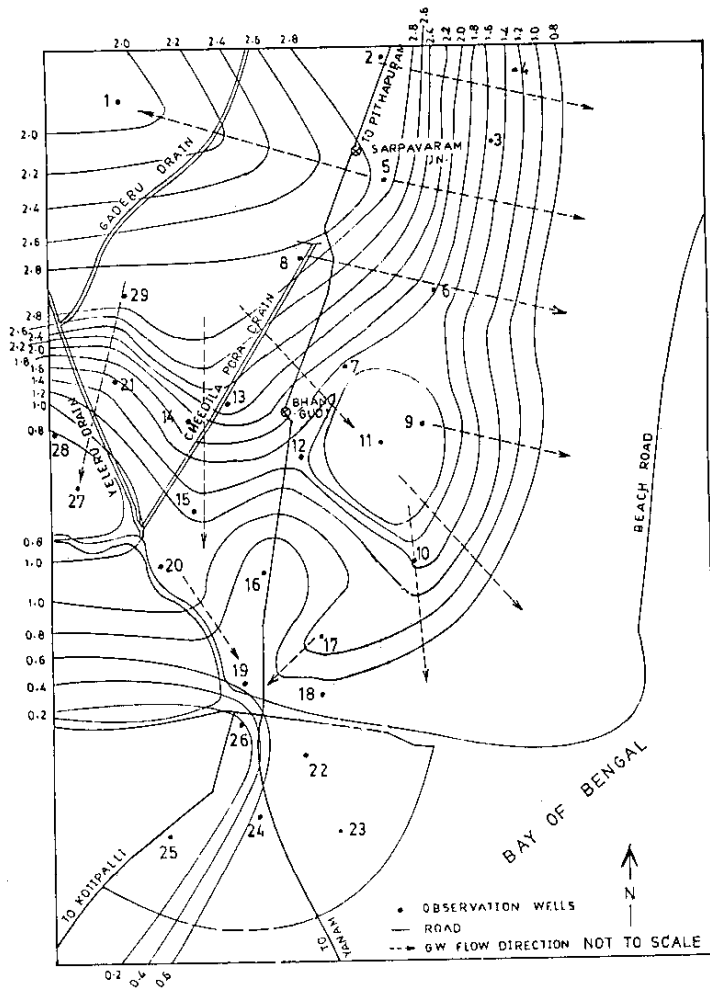
Fig. 7 Reduced groundwater table contours during premonsoon(June 96)
