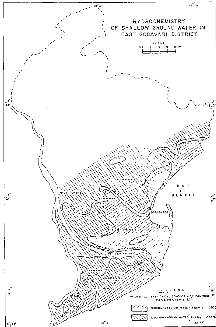
Fig. 3 Shallow groundwater Hydrochemistry of East Godavari district
