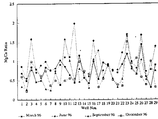
Fig. 17 Distribution of Hydrochemical ratios
