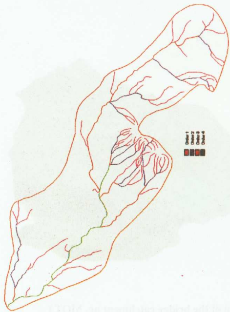
Fig. 10 Drainage network map of the bridge catchment no. MOT 4
