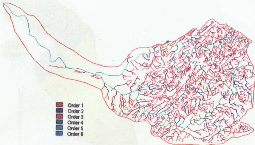
Fig. 8 Drainage network map of the bridge catchment no. MOT3
