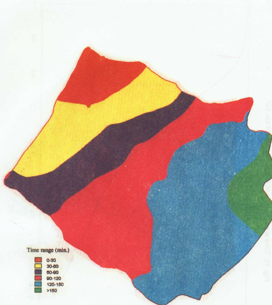
Fig. 12 Time area diagram of bridge catchment no. 527
