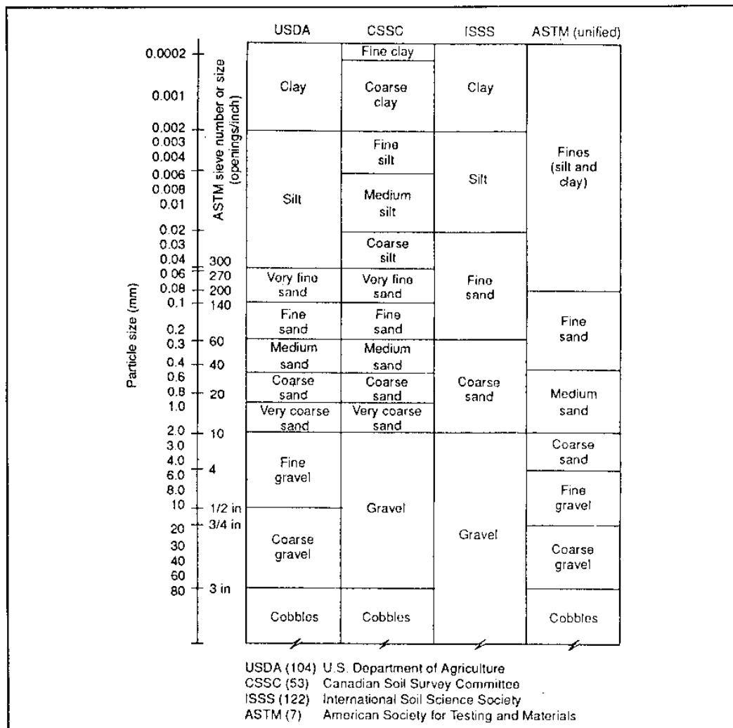
Figure 4.4: Particle size distribution ranges for various classification. (Source: Dravid, R. Maidment, 1992. Handbook of Hydrology, pp-5.3)
