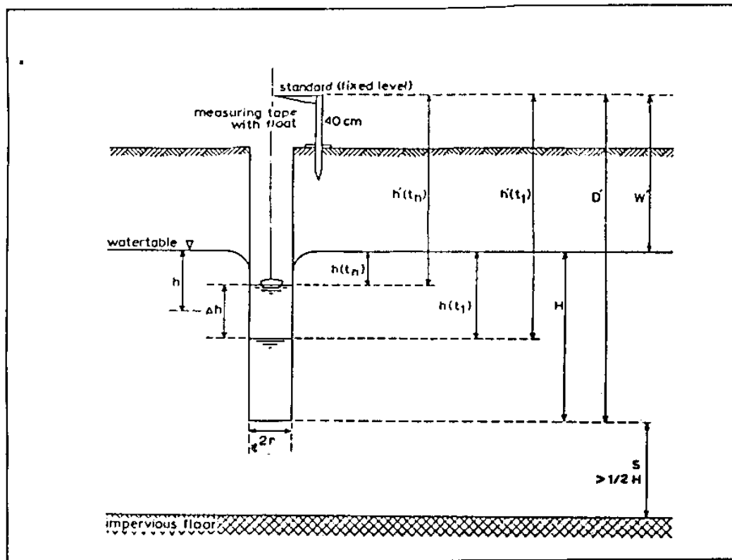
Figure 2.1: The Auger Hole method
