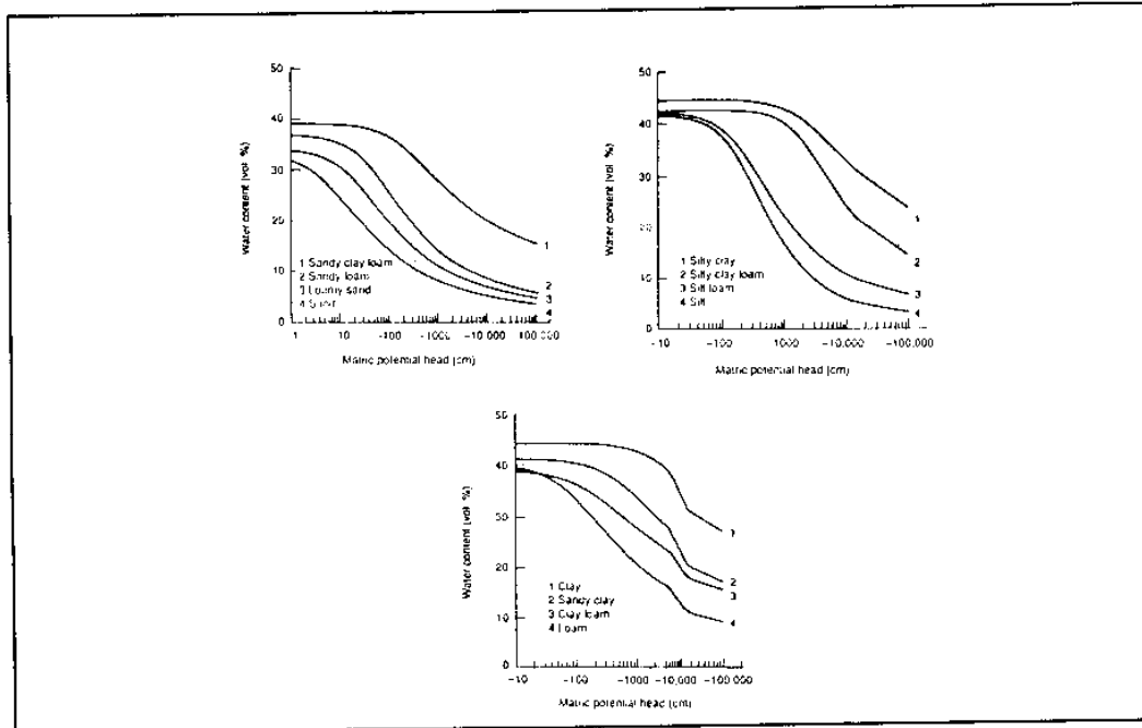
Figure 4.6: Water retention curves for USDA soil textures.
