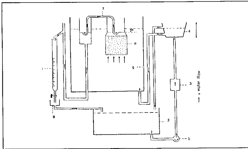
Figure 2.5: Working principle of ICW Laboratory Permeameter.
