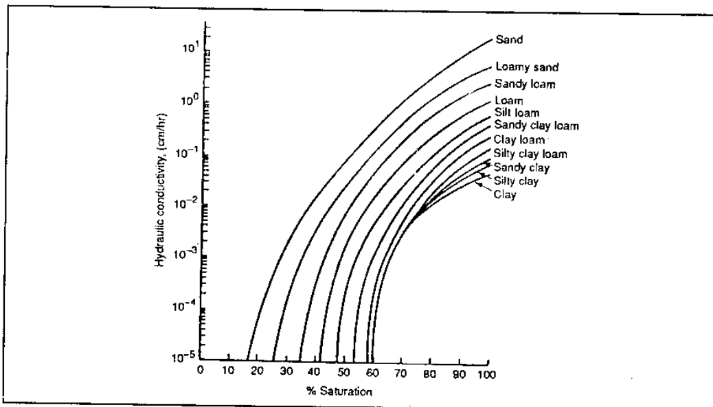
Figure 4.8: Hydraulic conductivity sorted by soil texture.
