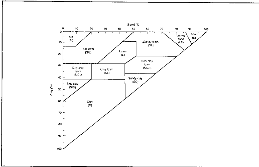
Figure 4.5: Soil texture triangle.
