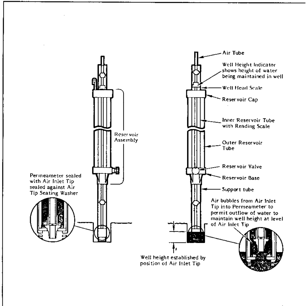
Figure 4.2: Different parts of a Guelph Permeameter.
