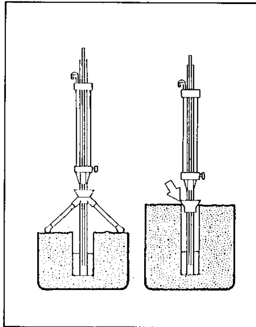
Figure 4.3: Permeameter placement.
