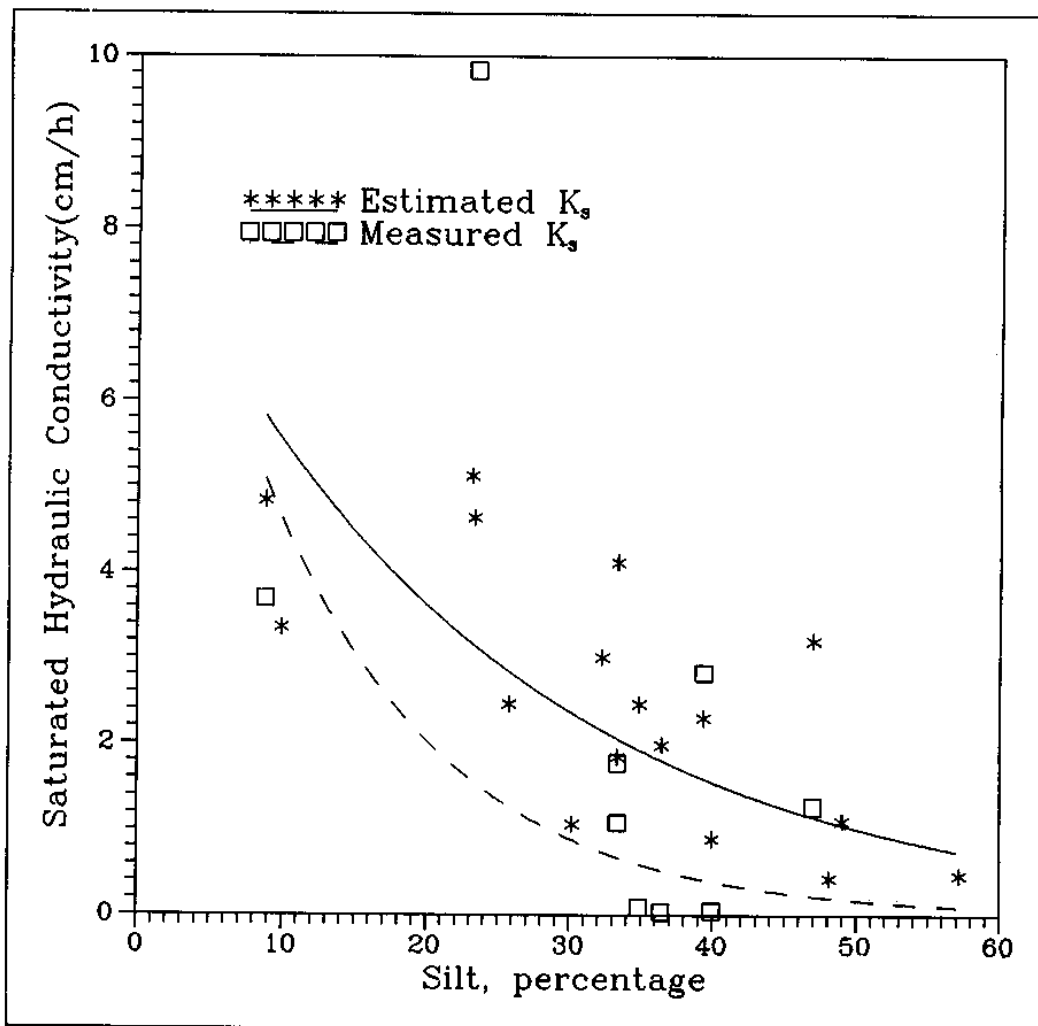
Figure 5.2: Silt Percentage v/s Saturated Conductivity Curve.
