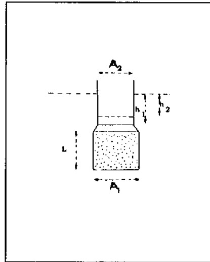
Figure 2.6: Reading by Falling Head method.
