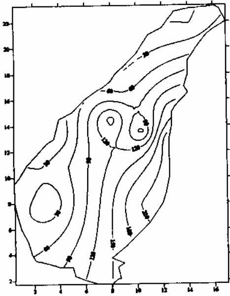
Fig.C-5: 9 hourly Isohyetal map of Pimpun Basin
