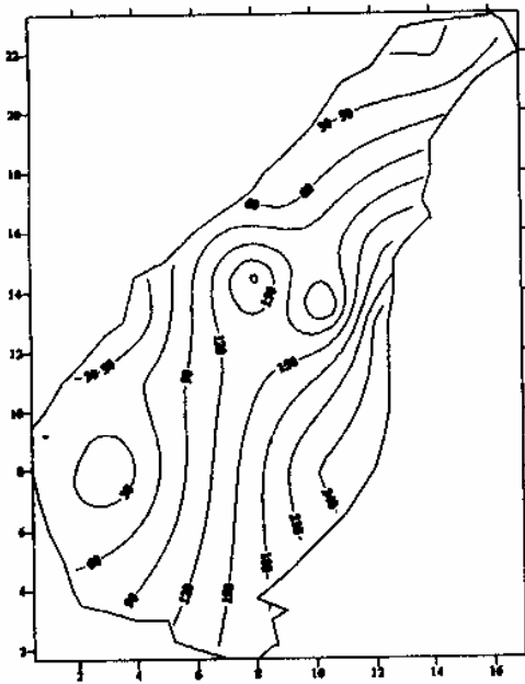
Fig.C-7: 18-hourly isohyetal map of Pimpun Basin
