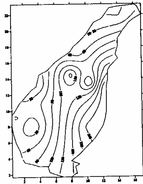
Fig.C-8: 24-hourly isohyetal map of Pimpun basin
