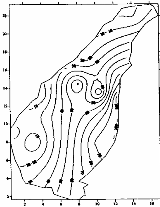
Fig.C-3: 3-hourly isohyetal map of Pimpun Basin
